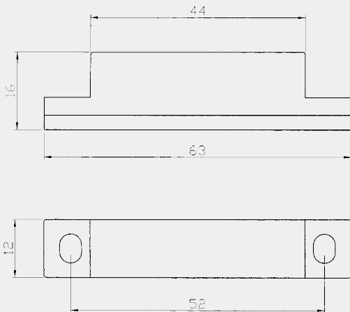
MAGNET
